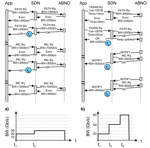
Fig. 2. Software-driven (a) and network-driven (b) models.
