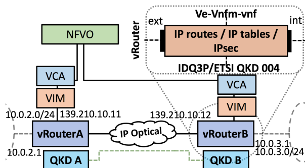
Fig. 1. Proposed architectural and node solutions
