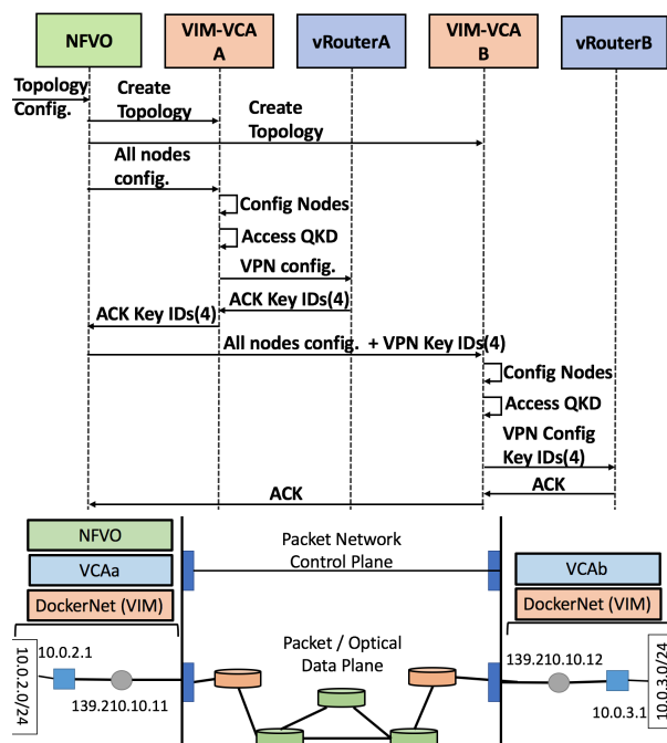
Fig 2 top) Workflow for the QKD-enabled VPN service automation; bottom) logical distribution of the scenario
